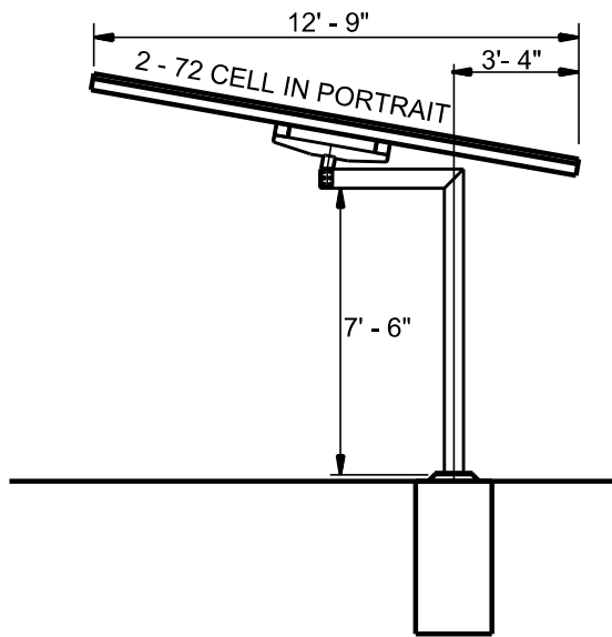
TYPICAL SECTION TILT UP
