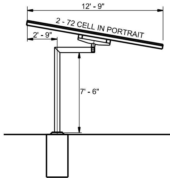
TYPICAL SECTION TILT DOWN
