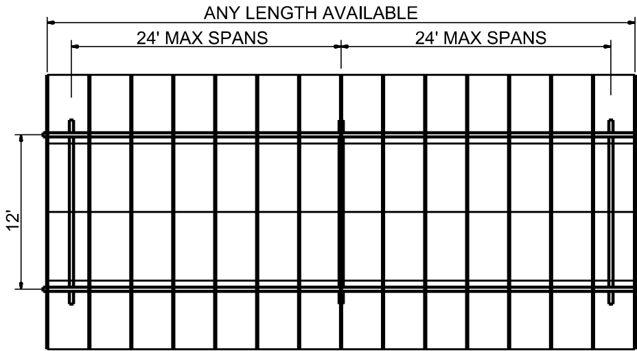
PLAN VIEW 4x 60 CELL IN PORTRAIT
