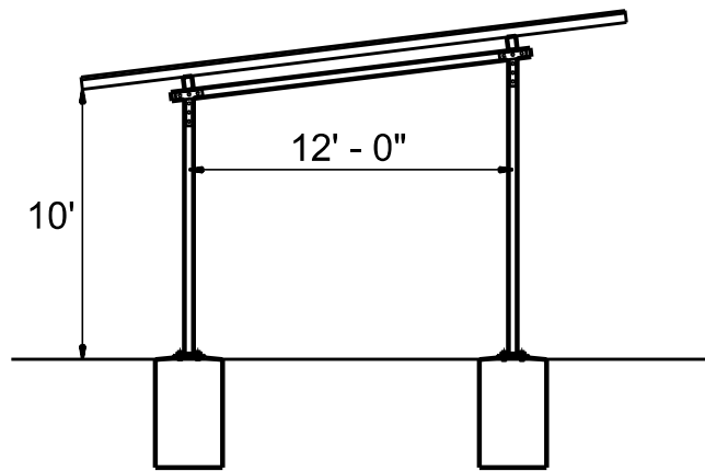
TYPICAL SECTION
